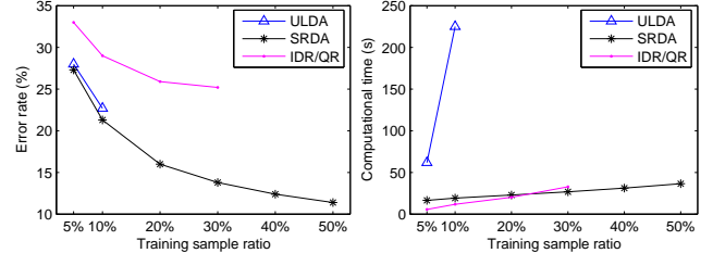
Fig. 4. Error rate and computational time as functions of number of labeled samples per class on 20Newsgroup.
