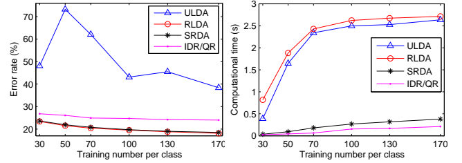
Fig. 3. Error rate and computational time as functions of number of labeled samples per class on MNIST.
